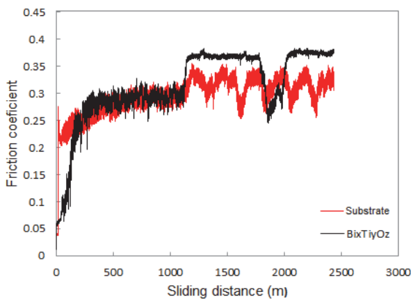
Figure 4. Representative curve of the wear coefficient the \text{Bi}_x\text{Ti}_y\text{O}_z coatings. Source: Authors.
