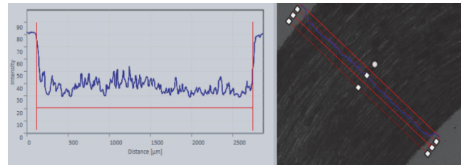
Figure 6. Width of the wear track on substrate SS 316L after 2420m. Source: Authors.
