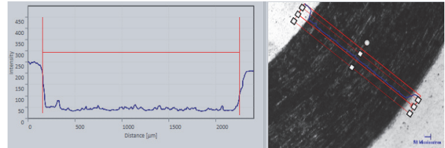
Figure 5. Width of the wear track on films of \text{Bi}_x\text{Ti}_y\text{O}_z after 2420m. Source: Authors.
