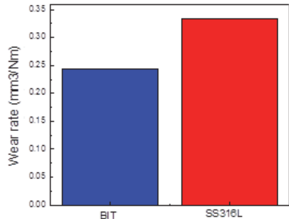
Figure 7. Calculation of the rate of wear after 2420m. Source: Authors.
